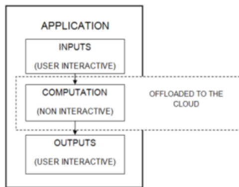
Fig 1: Partitioning of applications into interactive and non-interactive parts
